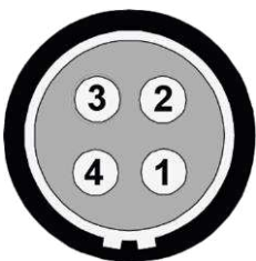
Figure 2: Pin assignment power output (socket view, device)
