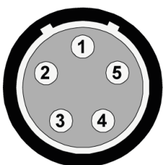
Figure 5: Pin assignment AUX (socket view, cable)
