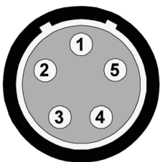
Figure 4: Pin assignment TRG trigger bus (socket view, cable)
