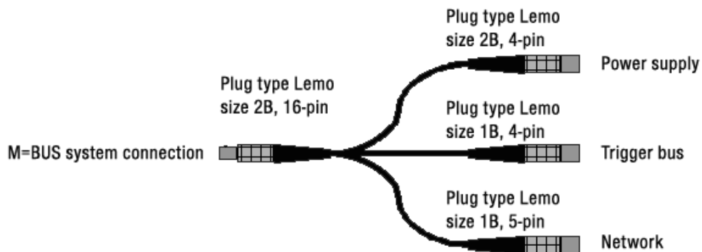
Figure 7: M=BUS Ethernet Gateway adapter cable
