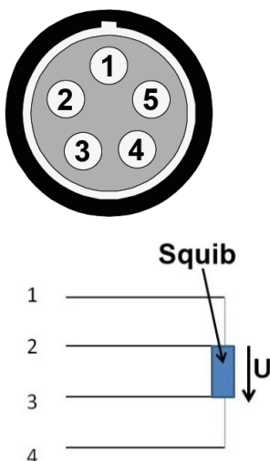
Figure 1: Pin assignment ignition output (socket view, device)
