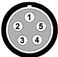
Figure 2: Pin assignment ignition channel (socket view, device)
