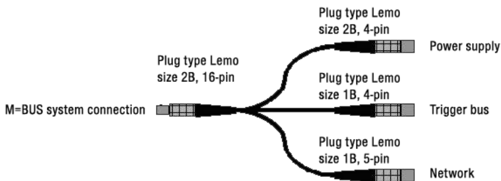
Figure 3: M=BUS Ethernet Gateway adapter
