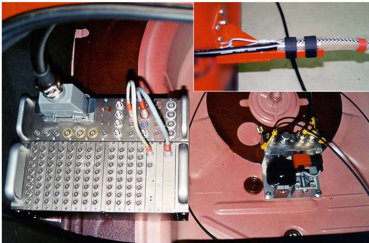
Sled with trailing cable connector box, NA33 System and hydraulic vehicle brake
